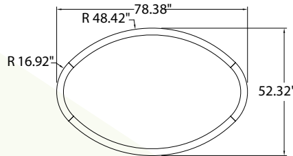
XTA | 2.0 Ellipse Recessed 78.38" Run Length 205.31"
