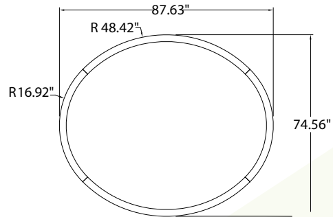
XTA | 2.0 Ellipse Recessed 87.63" Run Length 254.80"
